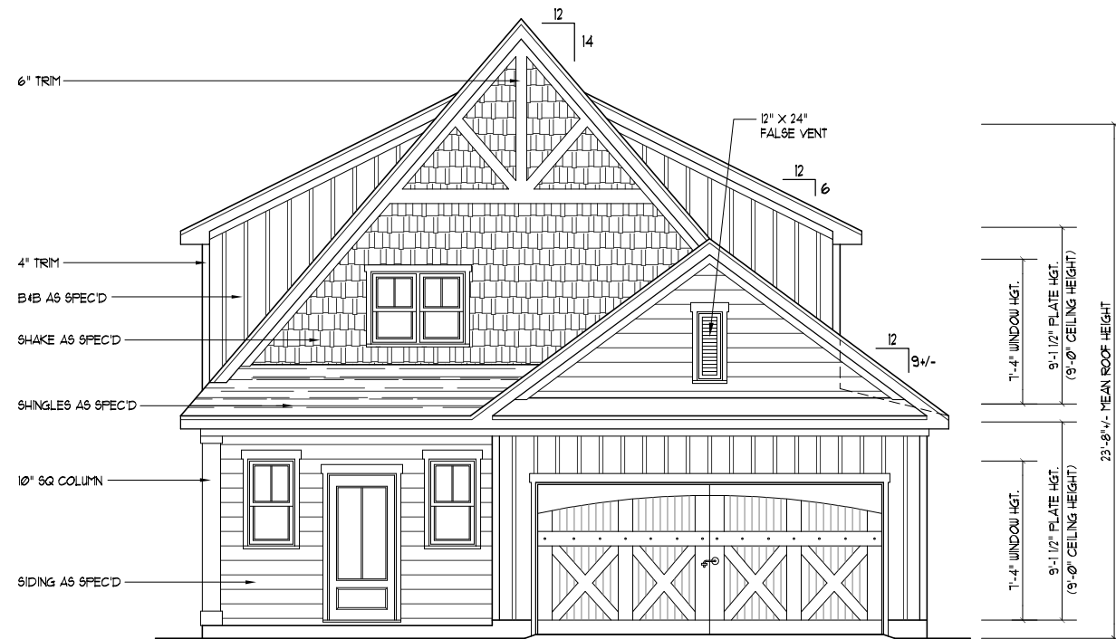
FRONT ELEVATION "C" SCALE: -----1/4" = 1'-0"
