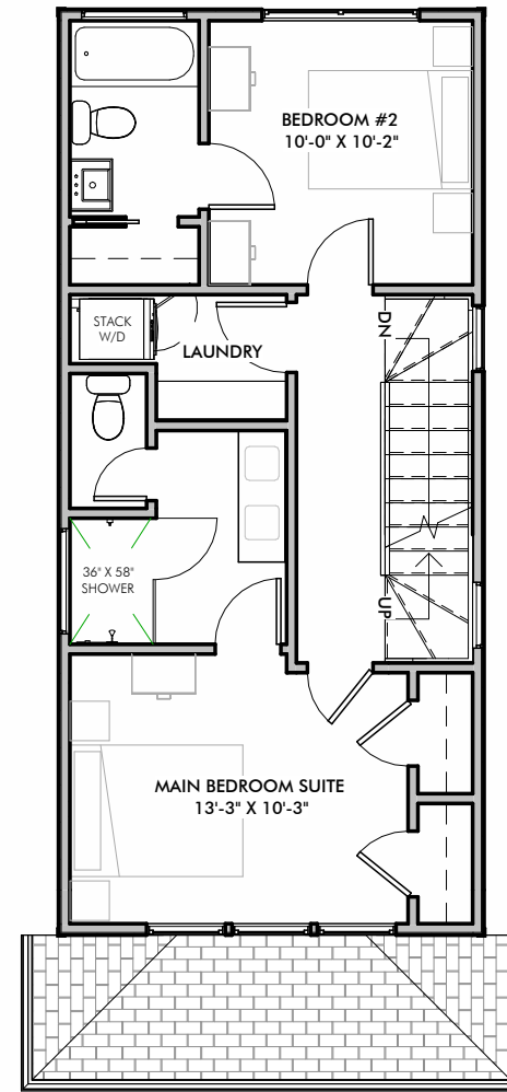
SECOND FLOOR PLAN 1/8" = 1'-0"
