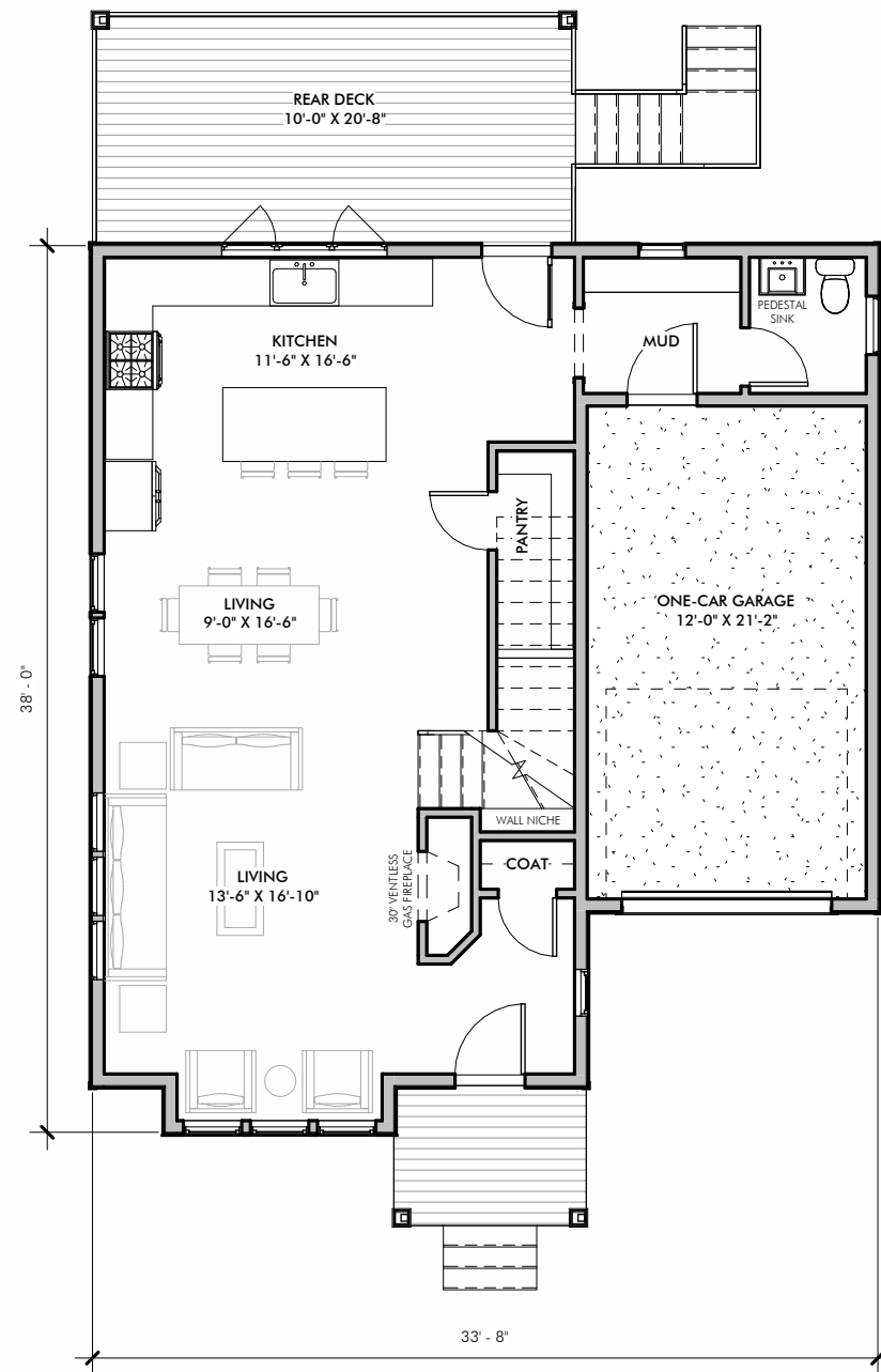
FIRST FLOOR PLAN 1/8" = 1'-0"
