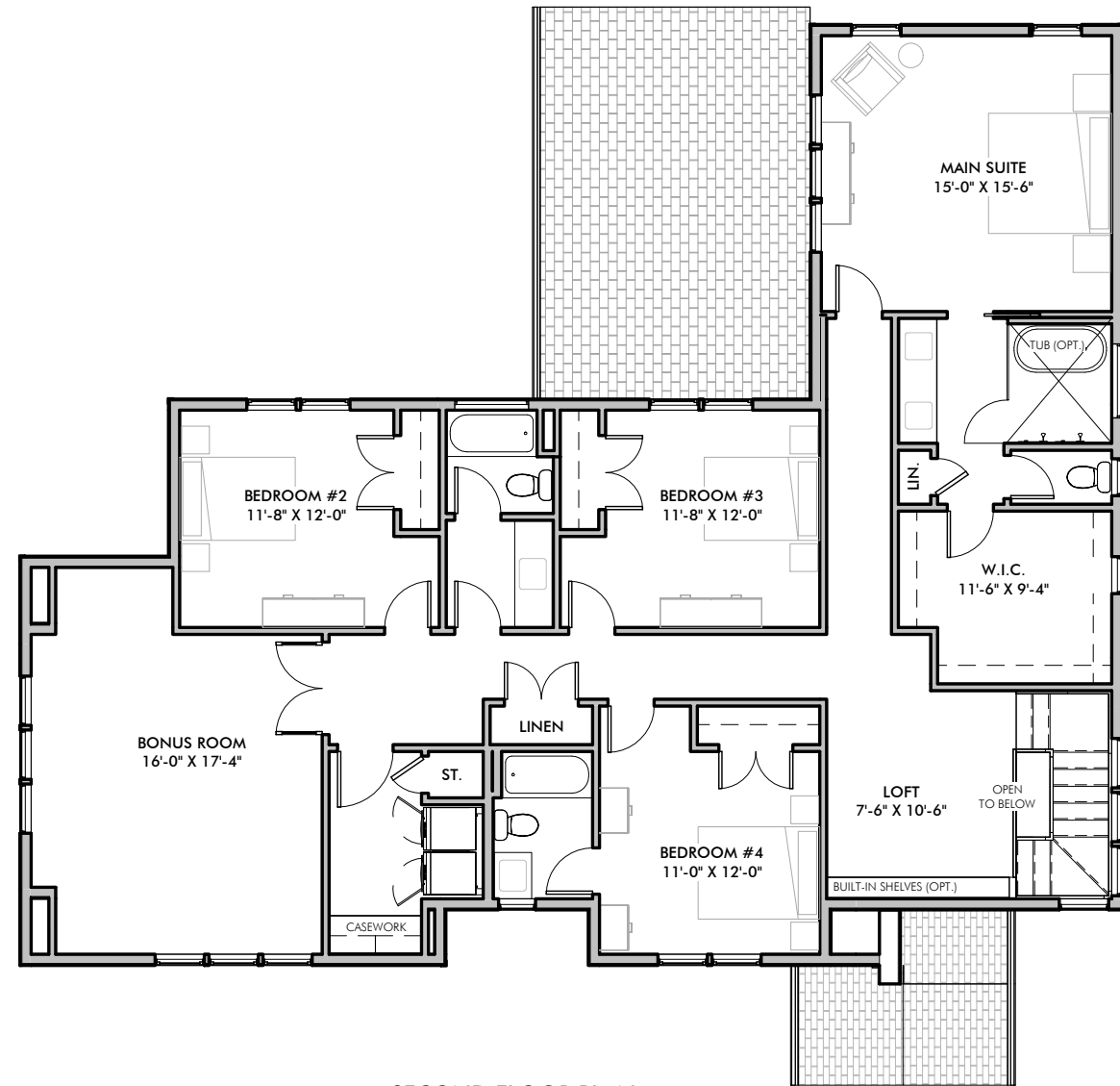
SECOND FLOOR PLAN 1" = 10'-0"
